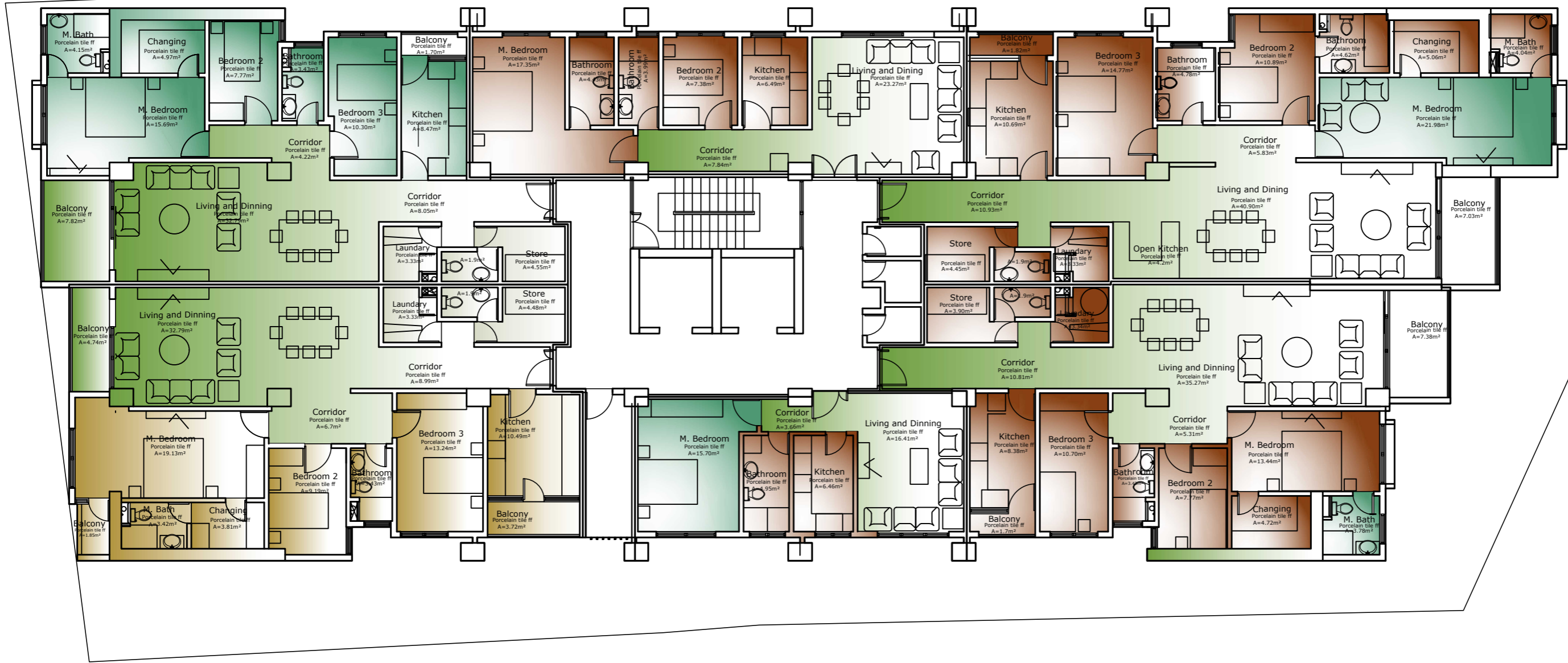
Typical 1st to 12th First to Floor Plan At Level +4.59 A=886.9m 2 Sc 1:100
